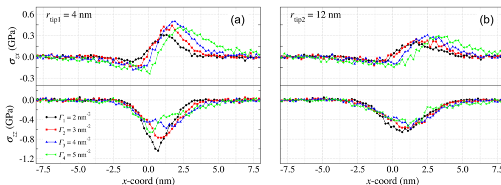
Figure 7. Spatial distribution of shear stress, \sigma_{zx} , and normal stress, \sigma_{zz} , for tip radii, r_{\text{tip}} = 4 nm (a) and 12 nm (b), at the highest load considered ( F_N = 30 nN). The sliding direction is +x . Standard deviations are smaller than the symbol size.
