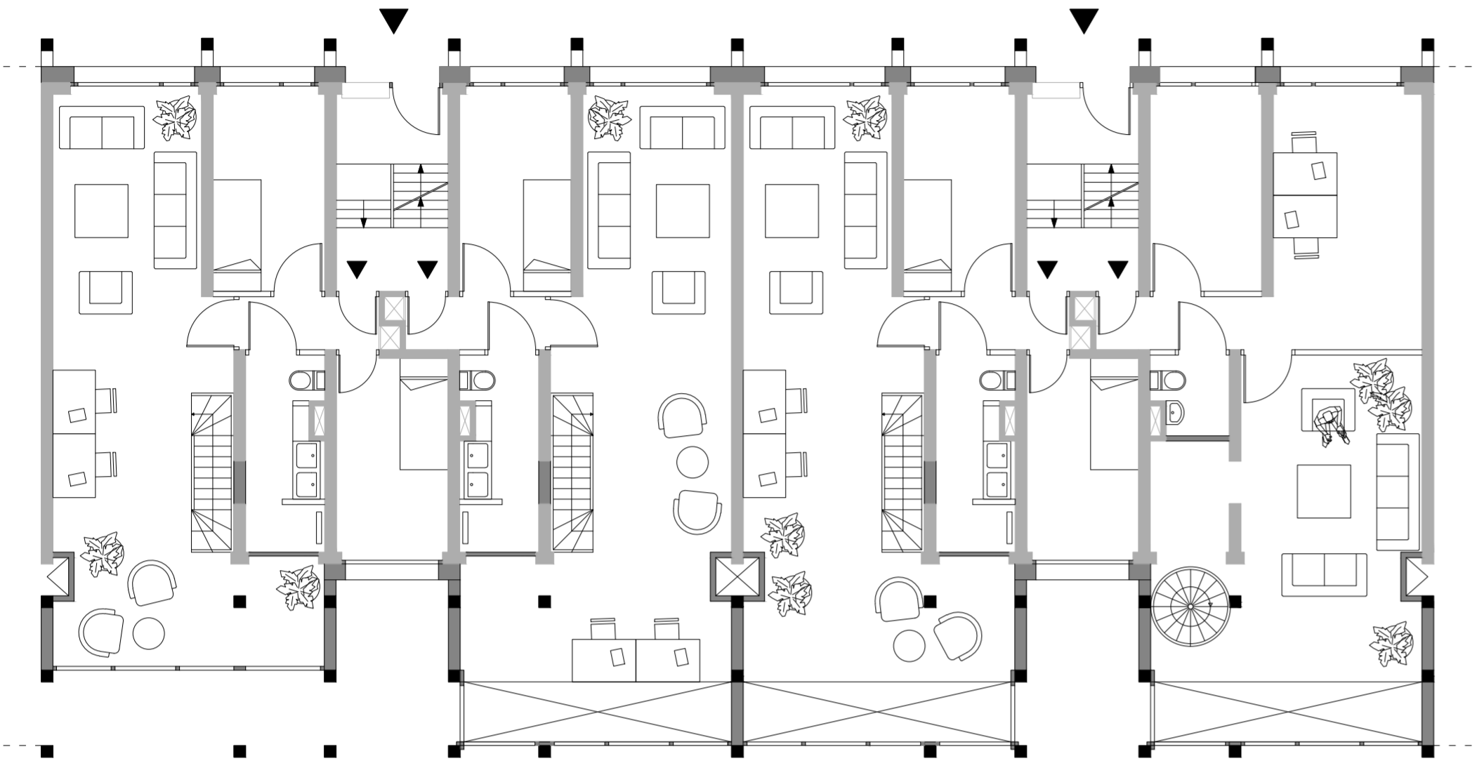
GROUND FLOOR
