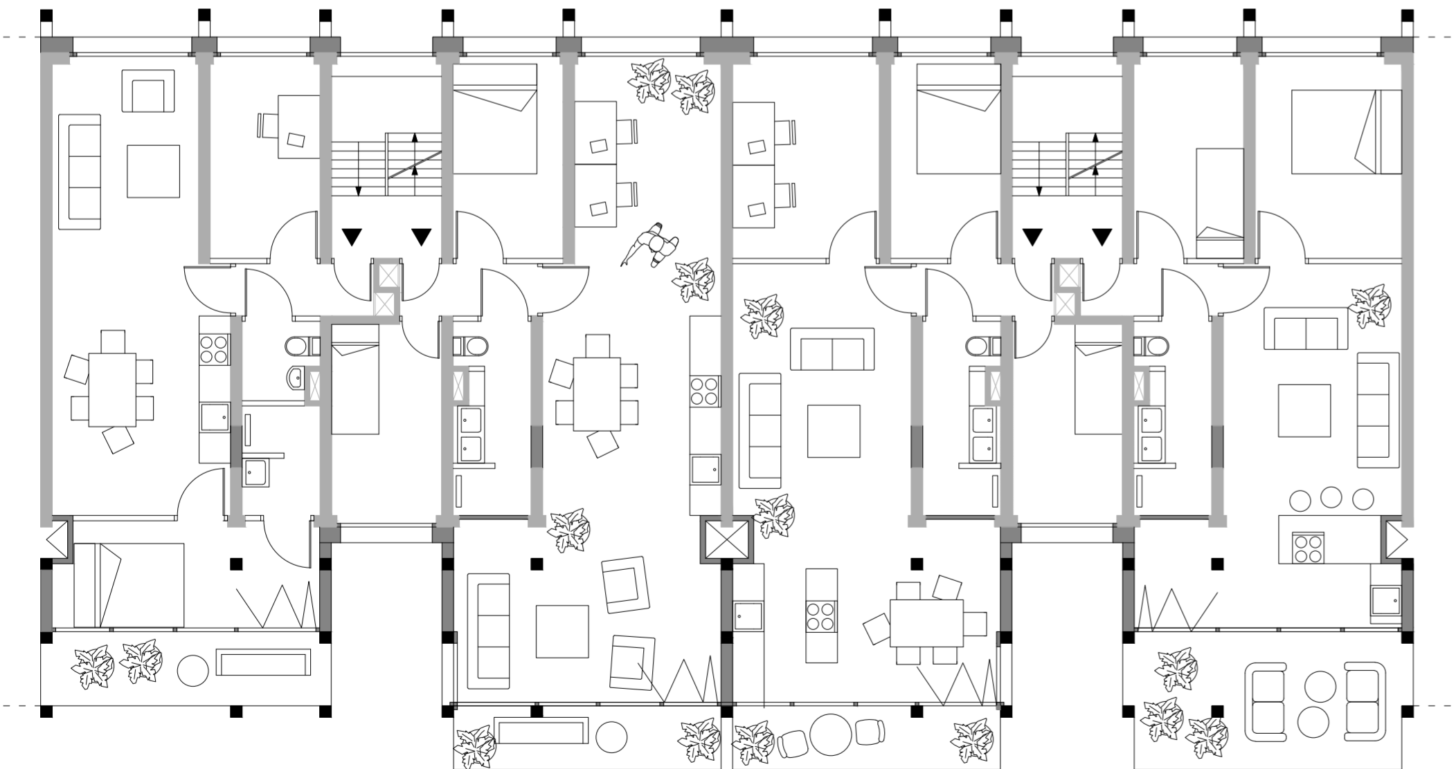
FIRST FLOOR
