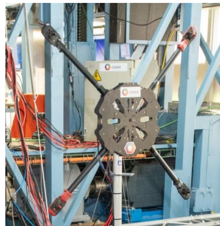
Figure 2. New 4 drone propellers for the inclusion of thrust and moments
