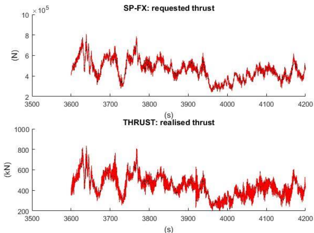
Figure 11. Comparison between actual thrust and set point
