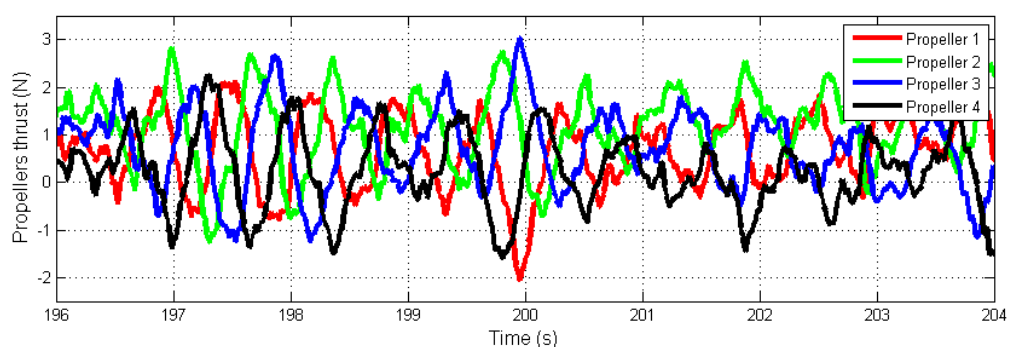
Figure 6. Thrust requested to the propellers for a production case with 16 m/s with one blade that fails to pitch and is fixed at 10^\circ
