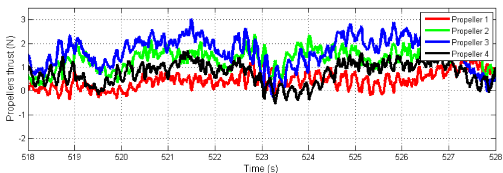
Figure 5. Thrust requested to the propellers for a production case with 16 m/s an the rotor yawed 30^\circ
