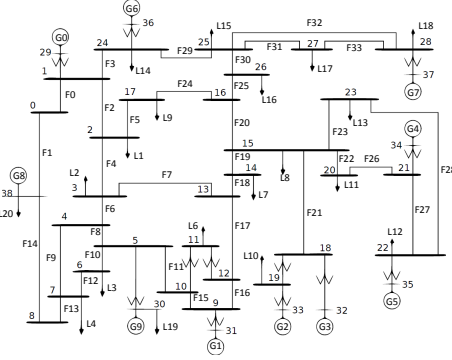
Fig. 6: IEEE 39 bus New England system.
