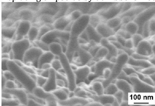
Fig. 4. Image of W fuzz showing nanorod ends widening first, rather than gradually thinning into a sharp tip. Reproduced from [4] with permission.
