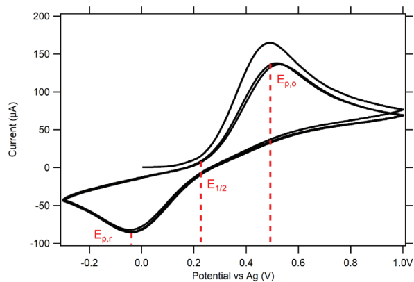
Figure A2.2. Example of a cyclic voltammogram of ferrocene in 0.1 M LiClO 4 in acetonitrile electrolyte solution, scanned at 50 mV/s. The oxidation and reduction peaks ( E_{p,o} and E_{p,r} respectively) are shown, as well as the half-wave potential ( E_{1/2} ).
