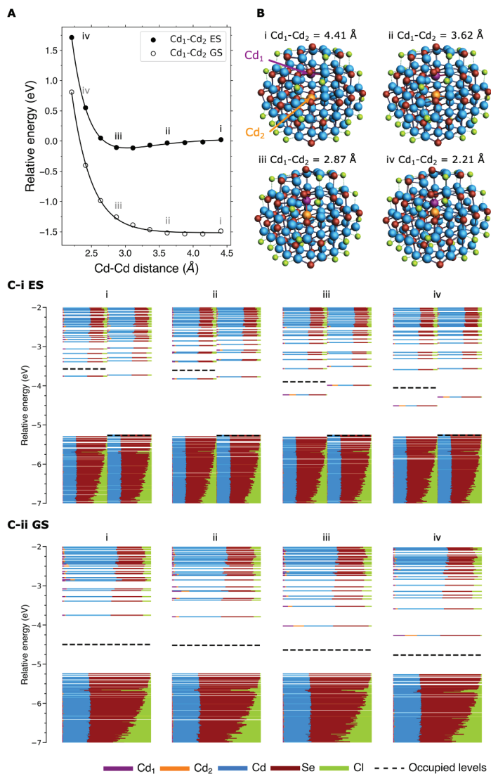
Figure A4.7. Comparison of the energy and DOS as function of the Cd-Cd distance in both the GS and ES. (A) Energy of the QD as function of the \text{Cd}_1\text{-Cd}_2 distance, in both the GS and ES (this figure shows the same data as Figure 4.4A in the main text). (B) Structure of the QD in the ES at varying \text{Cd}_1\text{-Cd}_2 distance. (C) The DOS for the same four \text{Cd}_1\text{-Cd}_2 distances, for both (i) the ES and (ii) GS. It can be seen that similar energy levels are pushed into the bandgap in both cases, but that there is no electron to occupy and thus stabilize the Cd level in the GS.
