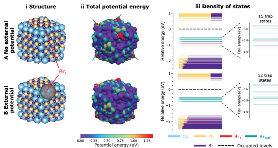
6 Figure 6.3. Effect of local potential on the energy of trap states (A) without and (B) with the application of an external potential. (i) Structure of model M8 and the location of the applied external potential around one of the five Br^- sites that give a deep trap, indicated as Br_1 . (ii) Total potential energy (i.e., the electrostatic potential generated by the nuclei and electrons plus the external potential, see Methods for details) of an electron at the NC surface (in eV). Blue colors correspond to a low potential energy, while red indicates a high potential energy. The location of Br_1 is indicated by the red arrow. The turquoise arrows indicate the other four Br^- sites that give rise to deep trap states. (iii) DOS, showing the contribution of the surface Br^- to the deep traps. Application of an external potential shifts the states from Br_1 into the VB, leaving 12 instead of 15 traps in the bandgap.
