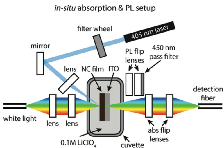
Figure A2.3. Schematic representation of the in-situ photoluminescence and absorbance setup.
