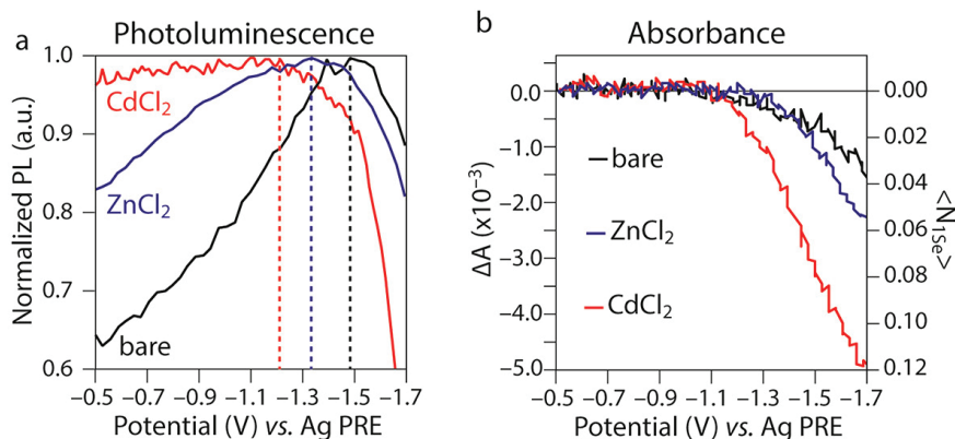
Figure 2.6. Comparison of in situ spectroelectrochemistry prior to and after metal chloride salt treatment. (A) Normalized PL intensity (at 691 nm) as a function of applied potential for CdTe NC films prior to (black line) and after metal chloride treatment (blue and red line). The PL drastically increases for untreated CdTe NCs before the band edge is reached when an electrochemical potential is applied (black line), whereas the PL is unaffected by the applied potential after CdCl 2 treatment (red line). The PL dependence of ZnCl 2 treated CdTe NC films lies in between. The onset of Auger recombination shifts to less negative potentials after treatment (indicated by the dashed lines). (B) Differential absorbance at the band edge (677 nm) as a function of applied potential for a bare CdTe NC film (black line) and CdTe NC films after ZnCl 2 (blue line) and CdCl 2 (red line) treatments. More electrons can be injected into the 1S c level after metal chloride passivation, and the maximum bleach of the 1S c level is not drastically shifted in potential by the treatments.
