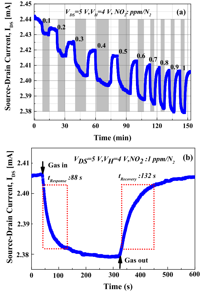
Fig. 12. Transient response of AlGaIn/GaN HEMT sensor to NO 2 gas concentrations at \sim 300^\circ \text{C} (a) 0.1-1 ppm. (b) Enlarged part of the response curve of 1 ppm.
