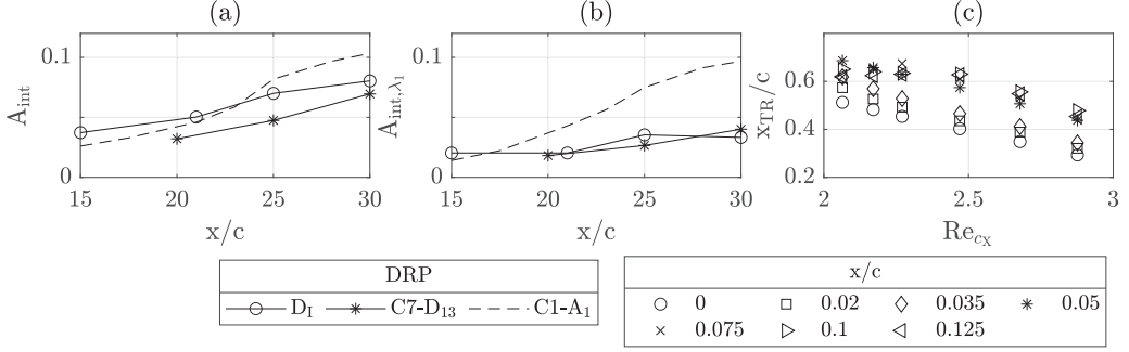
FIG. 13. Integral amplitude chordwise evolution for cases D_1 , C7-D_{13} , and C1-A_1 . (a) A_{int} ; (b) A_{int,\lambda_1} . (c) Transition front chordwise location at various Re_{cx} for DRP patches starting at various x_{DRP}/c .
