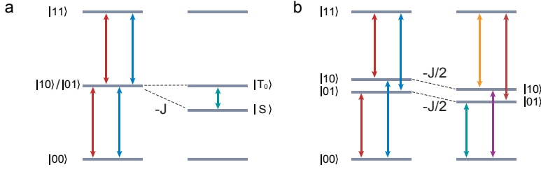
Fig. 2.2: Two-qubit energy diagrams affected by exchange interaction. a. When J \gg |f_1 - f_2| = 0 , the |T_0\rangle and |S\rangle states become the eigenstates. Under the Heisenberg Hamiltonian, this leads to the SWAP-class of two-qubit gates. b. When J \ll |f_1 - f_2| , |01\rangle and |10\rangle remain the eigenstates. The exchange interaction becomes an Ising Hamiltonian and thus enables the CPhase-class of two-qubit gates.
