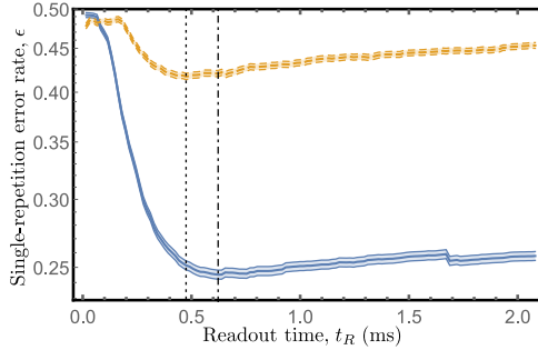
Fig. 6.4: Average single-repetition readout error rate \epsilon as a function of readout time t_R in the absence of added noise (solid blue line) and in the presence of added noise (dashed yellow line). The optimal readout time in the absence (presence) of added noise is indicated by the dot-dashed (dotted) line. In both cases, the shaded areas give the statistical uncertainty (see text). Finally, we note that the small discontinuity in the blue curve at t_R \approx 1.7 ms is a consequence of the finite histogram bin size and has no particular physical significance.
