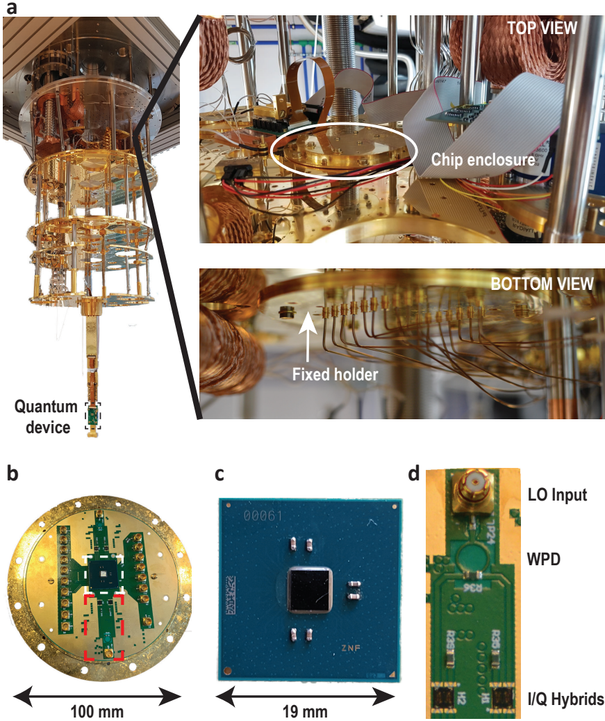
Fig. 8.7: Dilution refrigerator setup a. Location of the cryo-controller and the quantum device inside the dilution refrigerator (left). Top view and bottom view of the 3 K plate showing the mounted chip enclosure and the fixed holder for the enclosure respectively (right). b. Top view of the gold-plated annealed copper enclosure (without the lid) which is used to mount and thermalize the cryo-controller. c. Ball-grid-array (BGA)-324 package hosting the cryo-controller chip with on-package decoupling capacitors (highlighted as white box in b ). d. The Wilkinson power divider (WPD) splits the input LO power into two equal paths with half power in each implemented on a PCB. Discrete I/Q hybrids create the in-phase and quadrature phase component of the input LO are wire-bonded on the PCB for LO distribution between the different transmitters inside the cryo-controller (highlighted as red box in b ).
