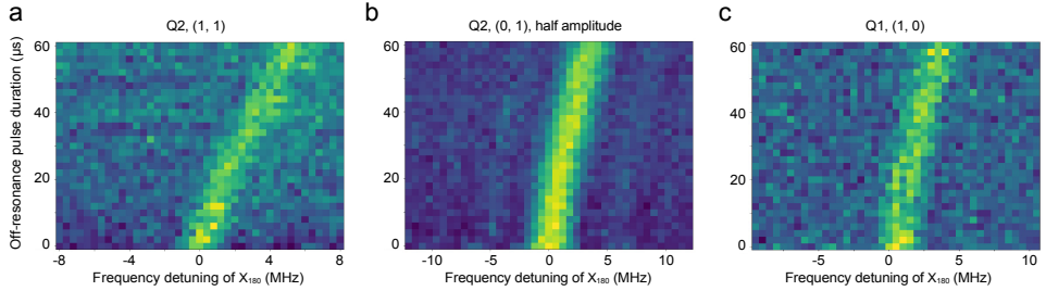
Fig. 9.2: a. Frequency shift of Q2 with a second qubit (Q1) present in the measurement. Q1’s frequency is detuned from Q2 by \sim +100 MHz and thus it’s not affected by the off-resonance pulse. b. Frequency shift of Q2 with the off-resonance pulse amplitude set to half of the X_{180} pulse amplitude. c. Frequency shift of Q1 measured in the absence of Q2.
