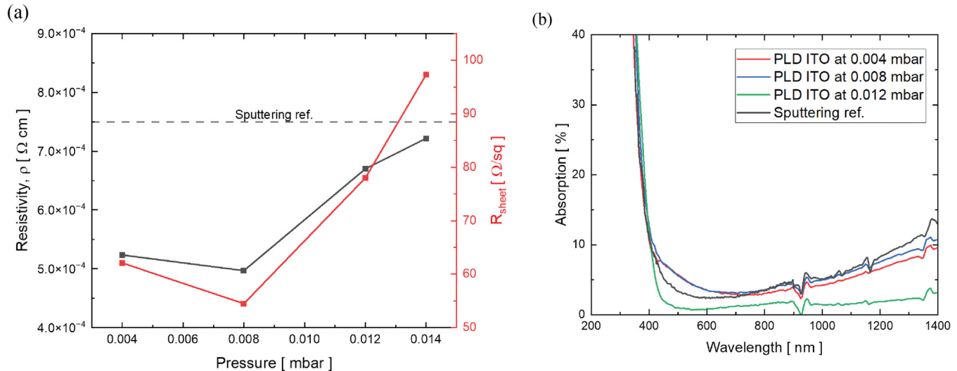
FIG. 7. Resistivity and R_{\text{sheet}} at varying oxygen pressures (0.004–0.014 mbar) (a) and absorption spectrum (b) of PLD ITO films. Opto-electrical properties of sputtered ITO reference are also included.
