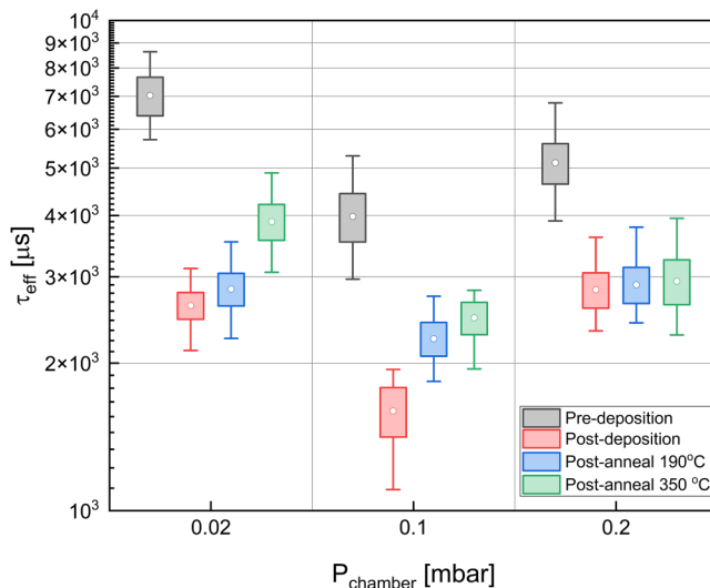
FIG. 5. Effect of P_{\text{chamber}} (0.02–0.2 mbar) on the surface passivation of 20 nm poly-Si contacts. ITO films are deposited at RT with O 2 /O 2 + Ar ratio = 0.2, repetition rate = 50 Hz, and laser fluence = 0.93 J/cm 2 .
