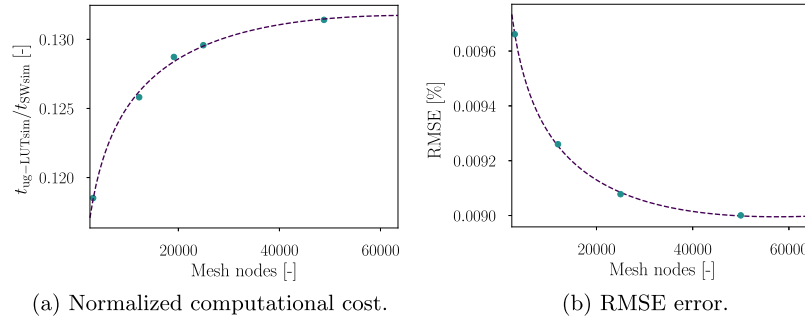
Fig. 7. 2D turbine cascade simulation results. (a) Normalized computational cost of the simulation employing the look-up table method ( ug-LUTsim ) compared to that of the simulation obtained using the Span-Wagner thermodynamic model ( SWsim ). (b) Relative mean square error (RMSE) of the Mach field from the SWsim and ug-LUTsim . The SWsim results are taken as reference.
