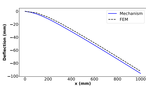
(a) Deflection: Rectangular cantilever
