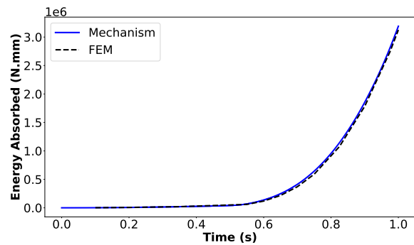
(h) Energy absorption: I-shaped simply supported
