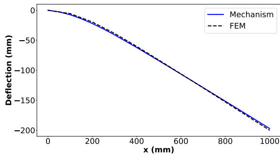
(e) Deflection: I-shaped cantilever
