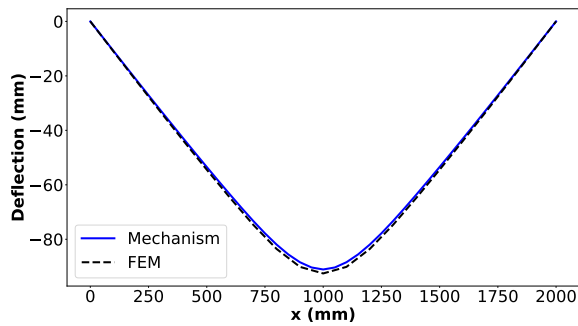
(c) Deflection: Rectangular simply supported
