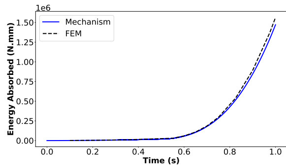
(f) Energy absorption: I-shaped cantilever
