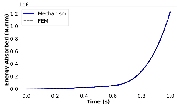
(b) Energy absorption: Rectangular cantilever
