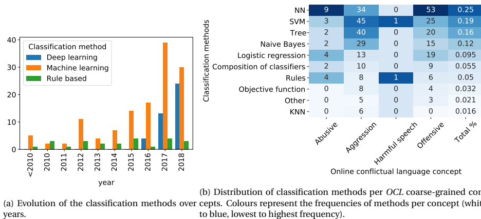
Figure 2.8: Quantitative analysis of the classification methods
