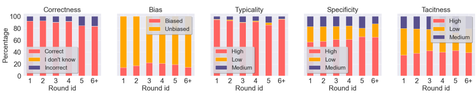
Figure 9.8: Bar plot illustrating the distribution of each dimension in the qualitative analysis of FindItOut in relation to the DA dataset, computed across different rounds.
