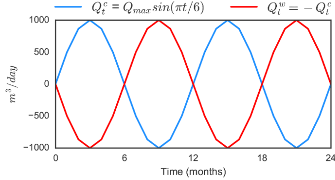
Figure 4: Seasonal ATEs injection/extraction flows
