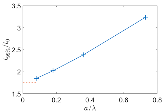
FIG. 5. (Color online) Saturation time of 99% t_{99\%} normalized by t_0 , against the particle radius a normalized by the gas mean free path \lambda . The red dashed line represents the normalized t_{99\%} in the free molecular regime, i.e., \lambda = \infty .
