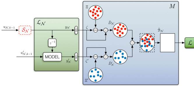
Fig. 4. Depiction of the proposed privatized, set-based communication scheme. By using a model of S_N dynamics, the agent \mathcal{L}_N can generate the value z' of the interconnection variable measurements under the hypothesis that S_N is driven by the adjacent input u'_N . By subtracting to both z' and to the true z two sets of samples of the measuring uncertainties, the sets \tilde{D}'_N and \tilde{D}_N are obtained. The hyper-box \tilde{B}_N is then computed as the smallest one containing both and its bounds are communicated to the agent \mathcal{L} .
