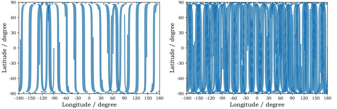
Figure 5. The subsatellite point coverage for 10 days (left) and 35 days (right) observation times. The sidereal period of Callisto is about 16.69 days.
