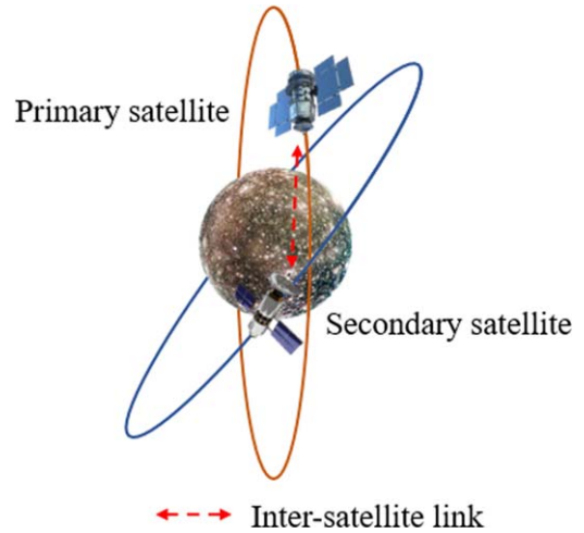
Figure 9. Orbital chart of the two satellites.
