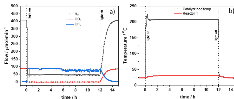
Figure 2. (a) \text{CH}_4 production rate as function of time for the \text{CO}_2 photomethanation without conventional reactor heating under 12.5 suns light intensity; (b) catalyst bed and reactor temperatures as function of time for the \text{CO}_2 photomethanation without conventional reactor heating under 12.5 suns light intensity. Reaction conditions: mixture of \text{H}_2:\text{CO}_2:\text{N}_2 (4.5:1:1) with a flow of 9:2:2\text{ mL}\cdot\text{min}^{-1} at 1.5 bar pressure (10 wt% \text{Ru}/\gamma\text{-Al}_2\text{O}_3 , 200 mg, AM 1.5 irradiance, 1 sun = 1\text{ kW}\cdot\text{m}^{-2} ).
