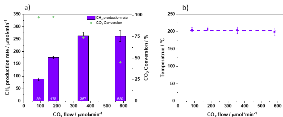
Figure 4. (a) CH 4 production rate as function of the reactant flow rate for the CO 2 photomethanation without conventional reactor heating under 14.4 suns light intensity without external heating; (b) measured temperature underneath the catalyst bed. Reaction conditions: mixture of H 2 :CO 2 :N 2 (4.5:1:1) at 1.5 bar pressure and 14.4 suns light intensity (10 wt% Ru/ \gamma -Al 2 O 3 , 200 mg, AM 1.5 irradiance, 1 sun = 1 kW·m −2 ).
