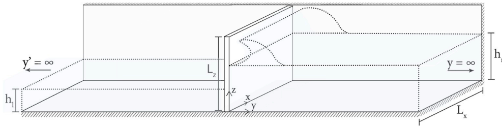
Fig. 1. Three dimensional overview of the plate model space.
