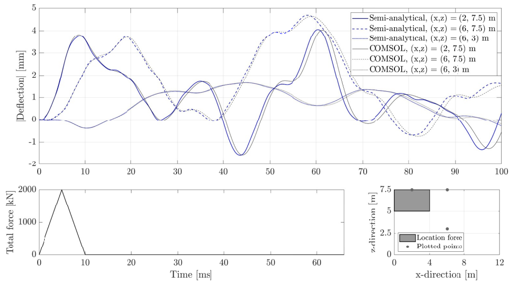
Fig. 13. The time-domain response of the gate immersed in fluid to a triangular peak load predicted by the semi-analytical model and COMSOL.
