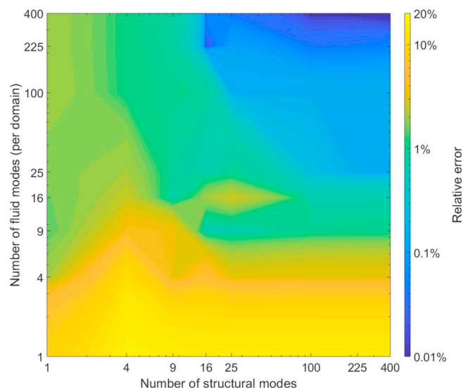
Fig. 12. The error in maximum plate stress found as a function of the number of structural and fluid modes taken into account relative to the result for both four hundred structural and fluid modes.
