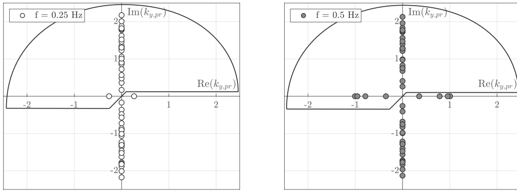
Fig. 7. The first 25 roots k_{y,pr} of the dispersion relation for the fluid domain at y < 0 ( h_l = 7 m) at frequencies 0.25 and 0.5 Hz.
