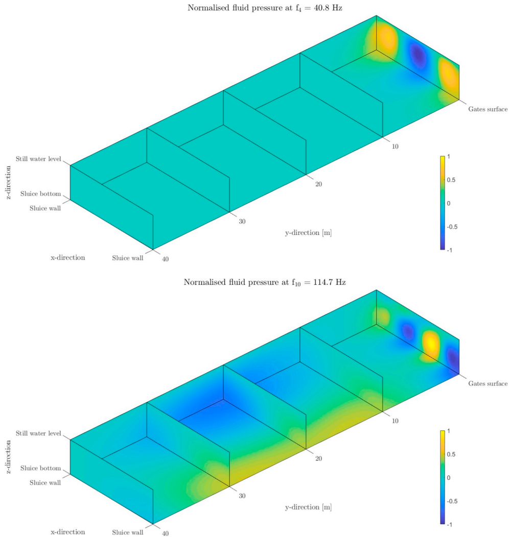
Fig. 9. Normalised absolute fluid pressure throughout the first 40 m of the sluice ( y > 0 ) at two of the resonance frequencies of the submerged gate.
