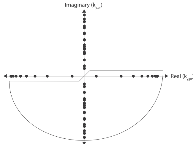
Fig. 2. Contour integration plot for the domain y > 0 together with the roots of the dispersion relation for a range of arbitrary parameters.
