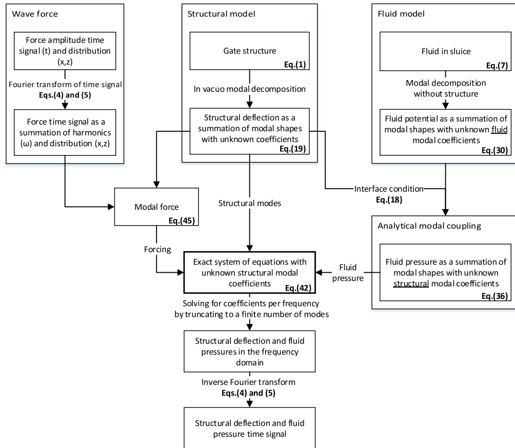
Fig. 3. Overview of the semi-analytical method. The result of the derivations in this chapter is the system of equations in Eq. (42).
