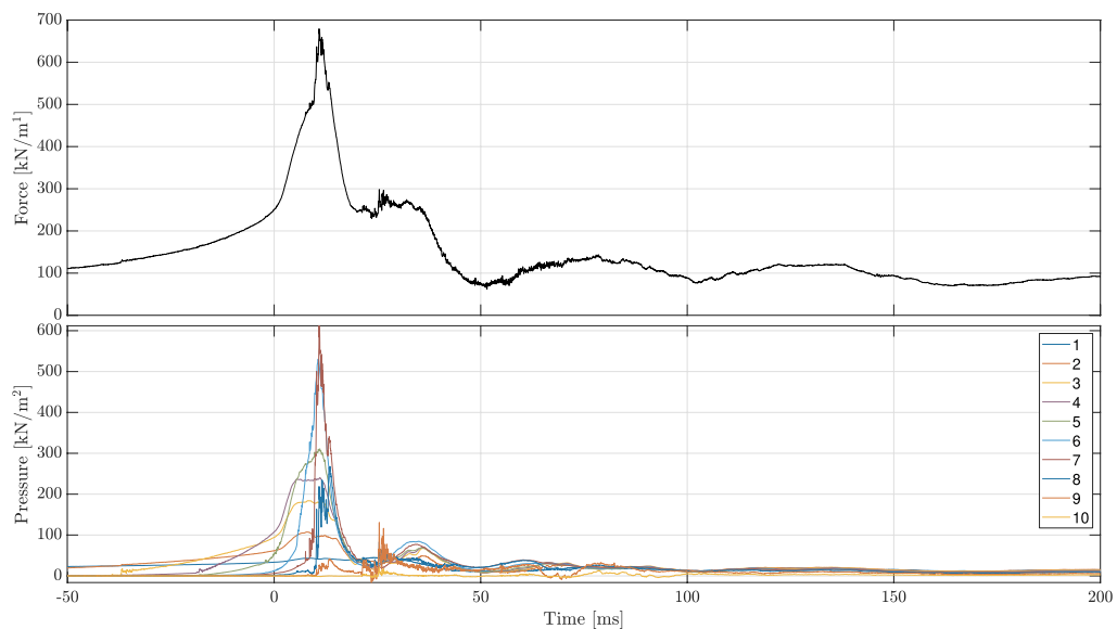
Fig. 5. Vertically integrated wave force and the wave pressure amplitudes for each of the 10 intervals over the vertical of the gate as defined in Fig. 4 over time. The maximum of the integrated wave pressure occurs at t = 10.88 \text{ ms} .
