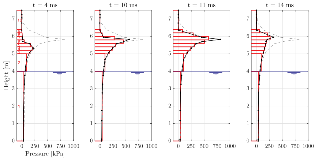
Fig. 4. Wave pressure over the vertical at four moments during impact. The dashed line denotes the envelope of the extreme pressures per location. In red the intervals are denoted that are used as input for the dynamic assessment. (For interpretation of the references to colour in this figure legend, the reader is referred to the Web version of this article.)
