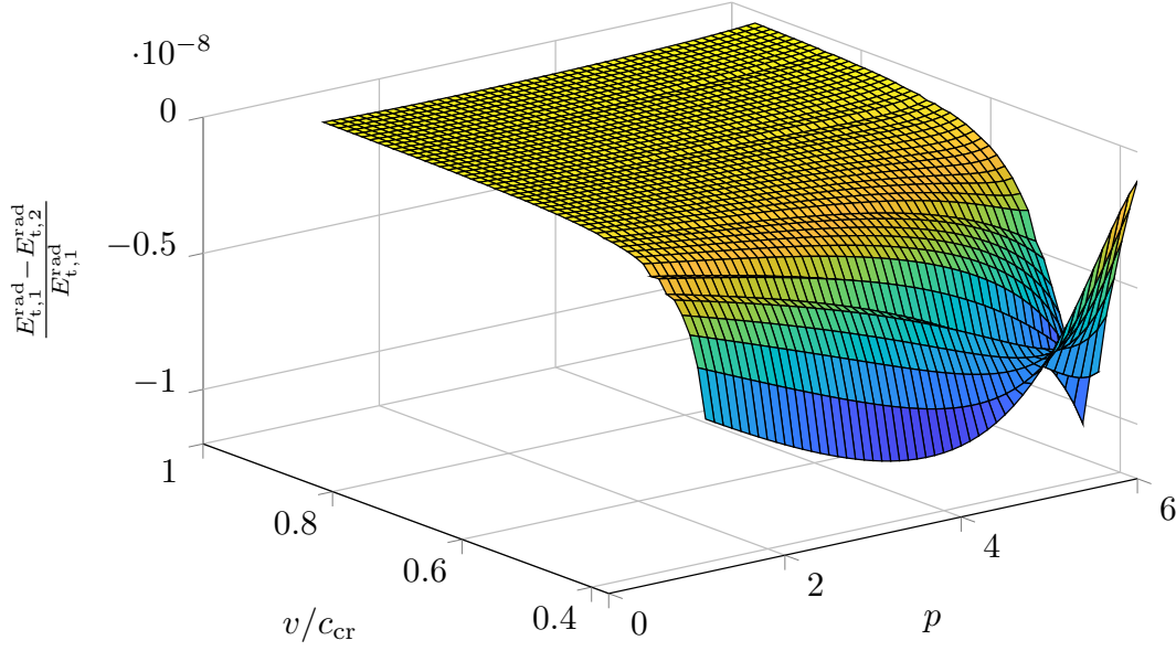
Figure 8: The relative difference in total energy radiated E_t^{\text{rad}} = E_1^{\text{rad}} + E_r^{\text{rad}} between the soft-to-stiff (subscript 1) and stiff-to-soft (subscript 2) scenarios for different relative velocities and stiffness ratios. As can be seen, the relative difference is almost null.
