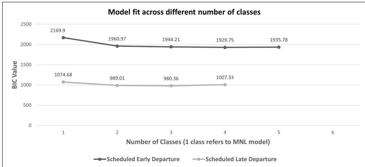
Fig. 4. BIC value for the MNL model and the LCCM.
