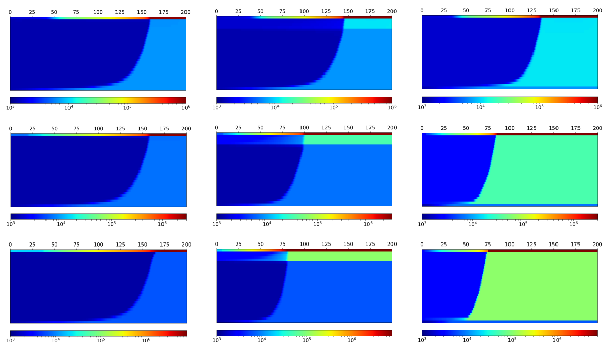
Figure 14 Total mobility ( \text{mD}/(\text{Pa} \cdot \text{s}) ) distributions in different layers at steady state. In all case, the lower-permeability layer is at the bottom. The plots illustrate different permeability ratios ( K_2/K_1 (first row), K_3/K_1 (second row), and K_4/K_1 (last row)) and different thickness ratios (1 m/29 m (first column), 5 m/25 m (second column), and 29 m/1 m (last column)), respectively.
