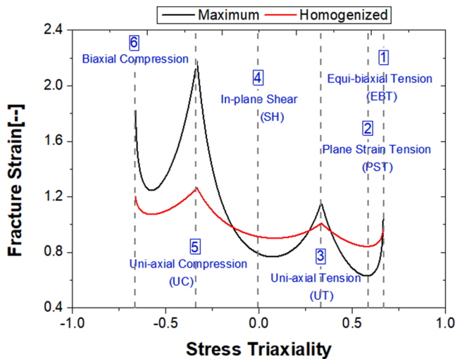
Fig. 12. Fracture strain vs. stress triaxiality exposed to plane stress states.
