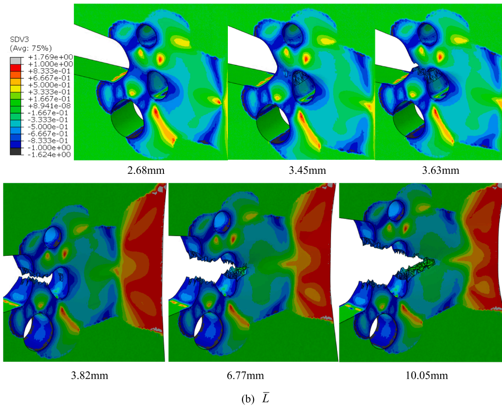
Fig. 27. Crack, stress triaxiality and lode parameter evolution of SFC specimen using maximum MCEPS.
