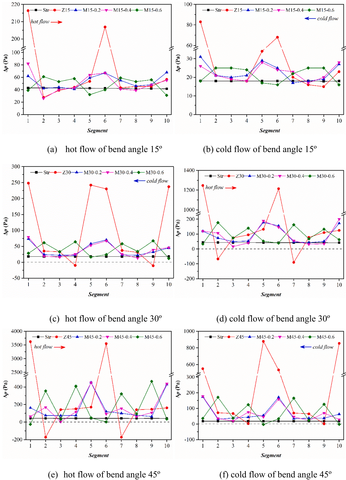
Fig. 7. The comparison of local pressure loss along the flow direction between the modified channel and the straight channel, zigzag channel. ( Re = 15000 , 6th pitch for wavy channels, 123 to 147.6 mm for straight channel).
