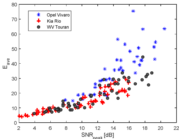
Figure 8. SNR_{peak}(E_{ave})
