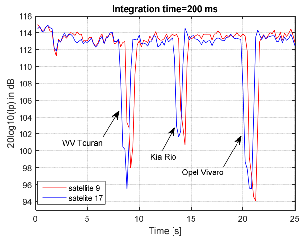
Figure 7. GPS shadows from satellites 9 and 17
