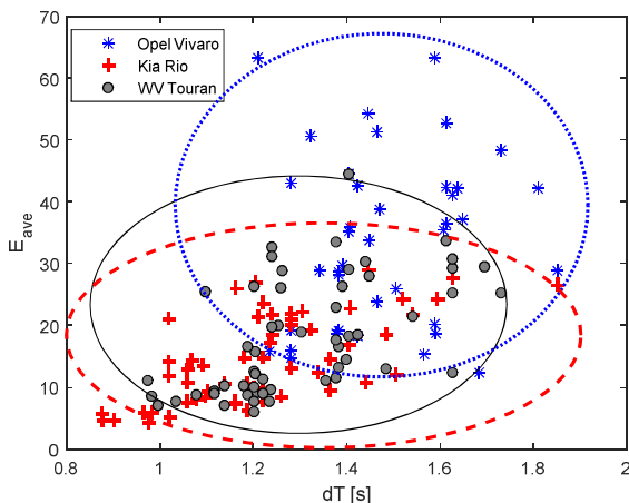
Figure 10. dT(E_{ave})
