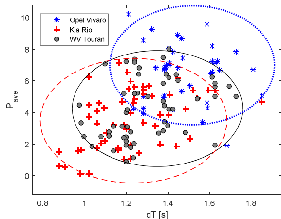
Figure 11. dT(P_{ave})
