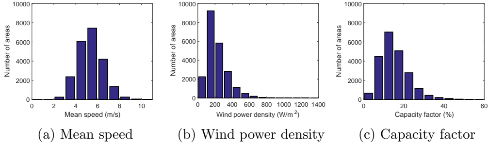
Figure 5: The characteristics of wind in Turkey
