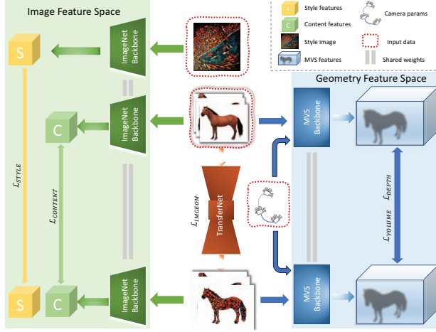
Figure 1. Our proposed network structure (MuViECAST) has three main components: Content-style feature extraction (green) operates on the image feature space for preserving the content and style. TransferNet performs image transformation. Geometry learning module (blue) operates on the geometry feature space for preserving the geometry.
