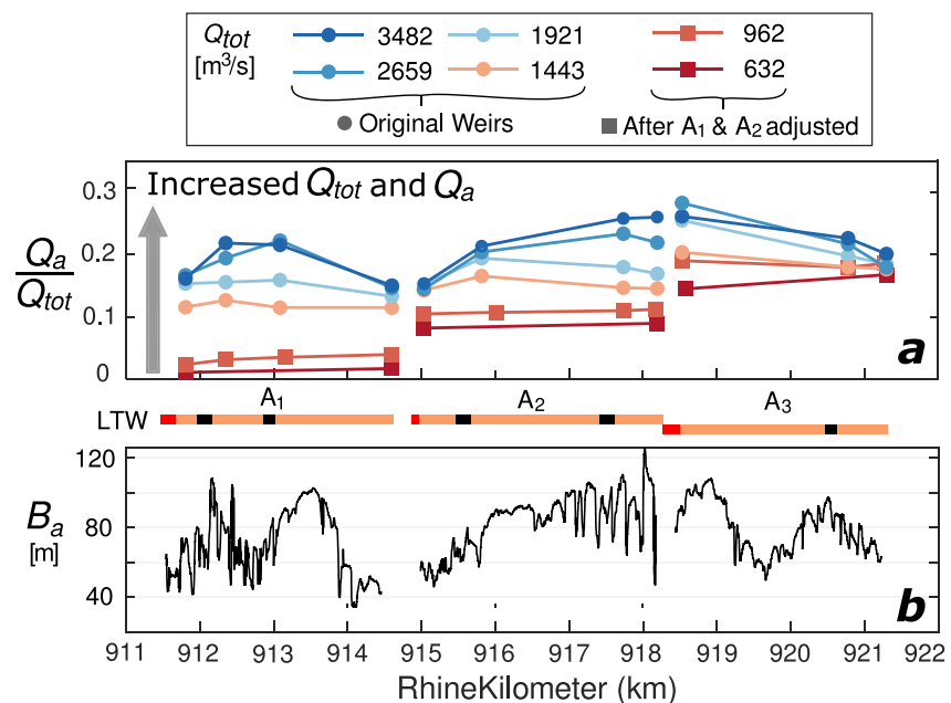
Figure 8. (a) Measured discharge in the auxiliary channels Q_a , normalized by the total discharge entering the study domain Q_{tot} ranging from about 600 to 3,400 m³/s. Discontinuities in the lines reflect the gaps between longitudinal training walls. Flows over 1,000 m³/s were measured with the original weir elevations, which had equivalent relative elevation. Flows lower than 1,000 m³/s were measured after A_1 and A_2 (RK 912–918) were raised, which reduced their discharge level. (b) Auxiliary channel width measured in all three auxiliary channels.
