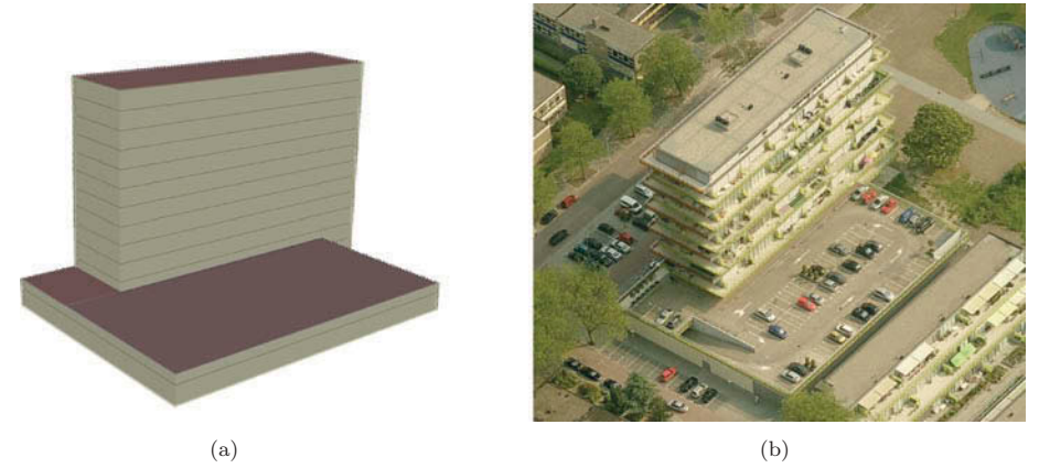
Figure 13. Comparison between: (a) a generated LOD2+ model and (b) the building from an aerial image taken from Bing Maps. Note how the short storey caused by a terrace is generated correctly in the LOD2+ model.
