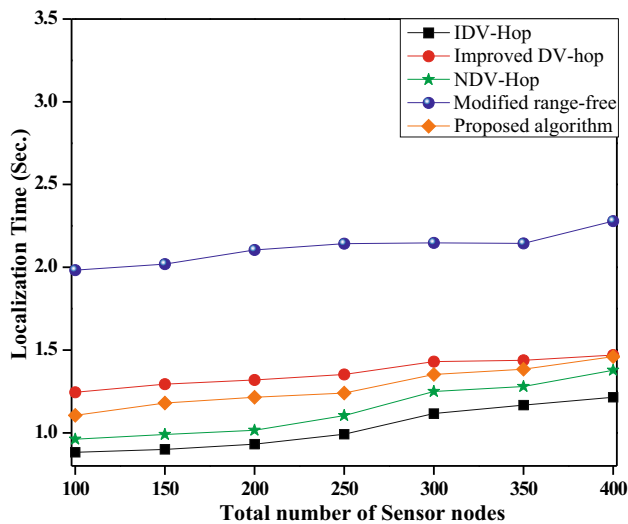
Fig. 14 Effect of total nodes on localization time
