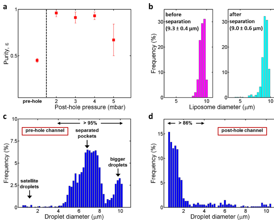
FIG. 2. Efficiency of the density-based separation technique. (a) Purity of liposomes obtained at different post-hole pressures. The pre-hole purity is also shown for comparison. The purity obtained is an average of at least three separate runs (number of particles analysed for each data set is > 1500 ). Error bars indicate standard deviations. (b) An example showing the frequency histograms of the liposomes in pre-hole (magenta, n = 1028 ) and post-hole (cyan, n = 541 ) channels. (c) Example of the size distribution of droplets in the pre-hole channel ( n = 2195 ). One can clearly see three discrete populations, belonging to—from left to right—smaller satellite droplets, droplets that are a result of the budding-off process from the liposomes, and bigger droplets that are formed as a result of instability at the production junction. The latter two populations (liposomes > 3.9 \mu\text{m} ) make up more than 95% of the population. (d) Example of the size distribution of the contaminating droplets in the post-hole channel ( n = 540 ), after the separation takes place. More than 86% of the droplets are below 3.9 \mu\text{m} , the cut-off value used for the purity analysis (see main text).
