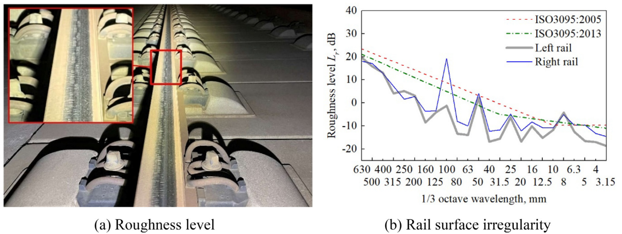
Fig. 13. Verification of rail surface irregularity at the track site C1.
