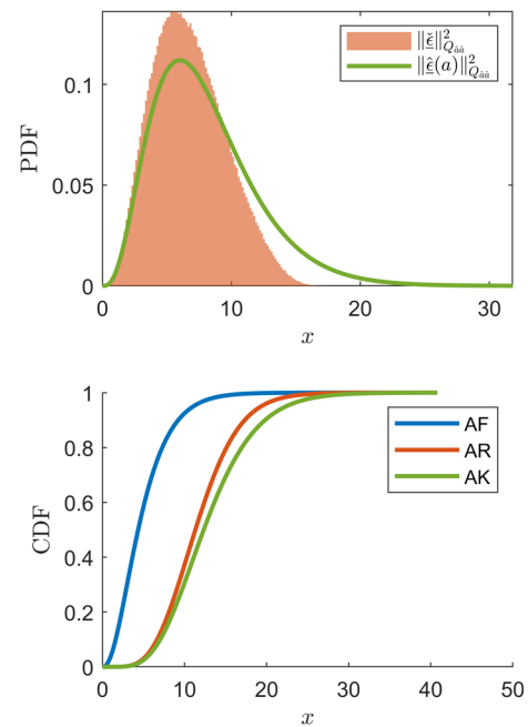
Fig. 6 (Top) \mathcal{H}_0 -PDFs of \|\check{\epsilon}\|_{Q_{\hat{a}\hat{a}}}^2 and \|\hat{\epsilon}(a)\|_{Q_{\hat{a}\hat{a}}}^2 ; (Bottom) \mathcal{H}_0 -CDFs of the AF-, AR- and AK-detector. The underlying model is a dual-frequency GPS model having a 62% ambiguity success rate
