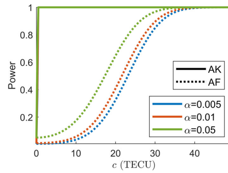
Fig. 4 AK- and AF-power function curves for ionosphere detection as function of iono-delay in TEC units, for different false-alarm probabilities (levels of significance \alpha ), based on a single-epoch, dual-frequency L1/L5 GPS model, with \sigma_p = 50\text{cm} and \sigma_\phi = 5\text{mm}
