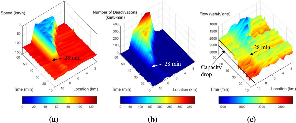
Figure 7 The relations among congestion pattern and number of deactivations. An example in the 60% CACC scenario with a 1200 veh/h on-ramp demand.
