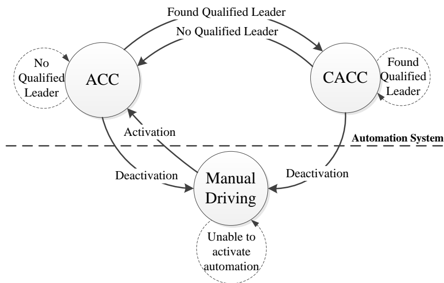
Figure 3 Switching paths between manual driving, ACC and CACC.
