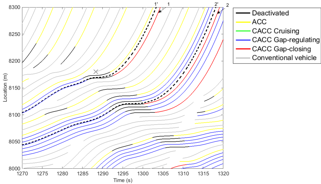
Figure 10 Virtual CACC vehicle Trajectories showing the increased large following gaps by CACC deactivation.
