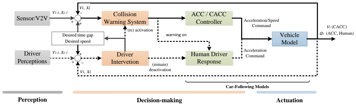
Figure 1 Conceptual longitudinal model for CACC vehicles in simulations.
