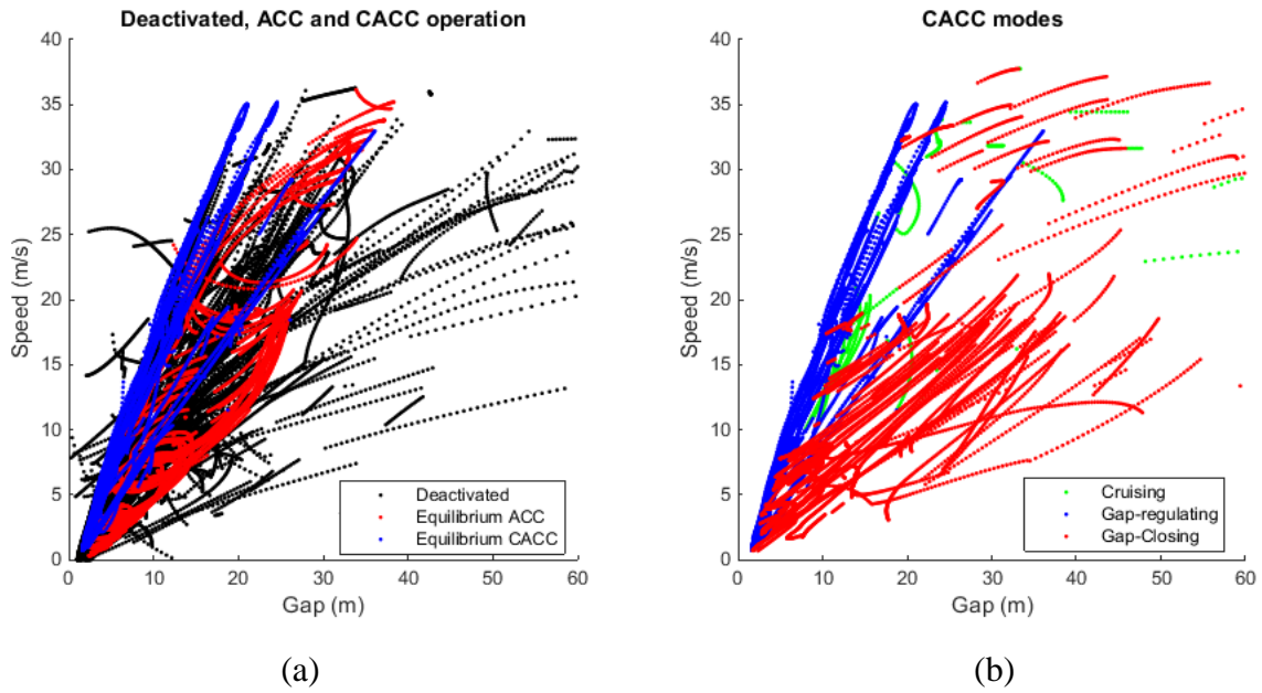
Figure 9 The Speed-Gap plot for manual driving, equilibrium ACC and equilibrium CACC operation (a); The Speed-Gap plot for Cruising, Gap-regulating and Gap-closing mode under CACC operation (b).
