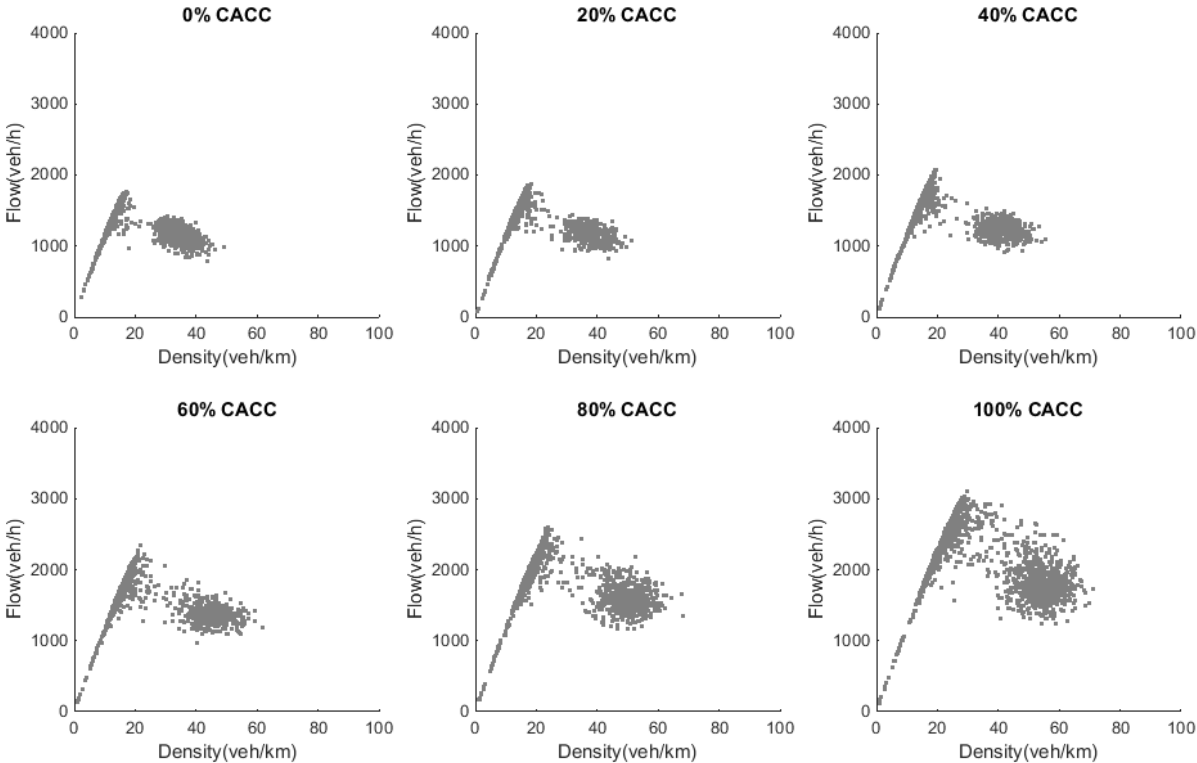
(a) Flow-Density plots with CACC MPRs
