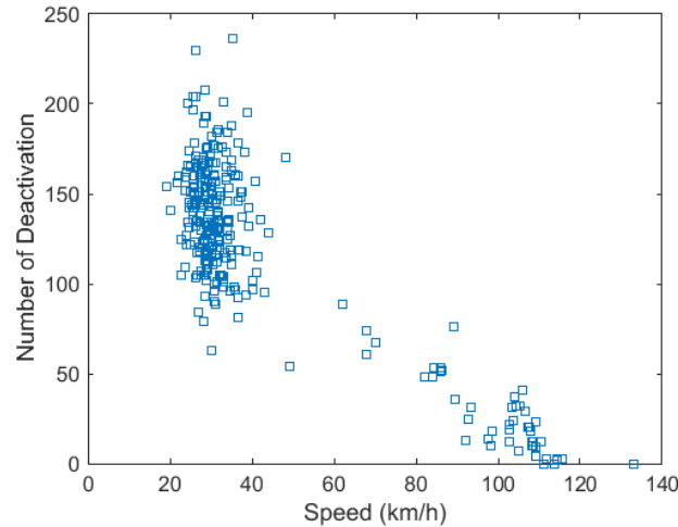
Figure 8 Plot of speed reduction and numbers of deactivation within 8-9 km. Data from simulation runs of the 60% CACC scenario with a 1200 veh/h on-ramp demand.
