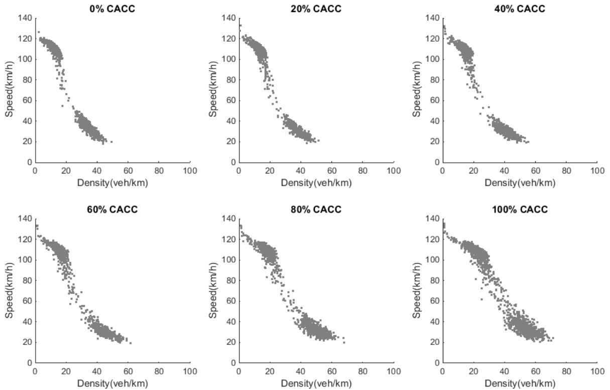
(b) Speed-Density plots with CACC MPRs
