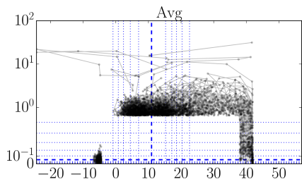
Figure 6. Illustrative plots for visually identifying outliers (see text for an explanation): FINO1 72 m ambient temperature data ( ^{\circ}\text{C} ).
