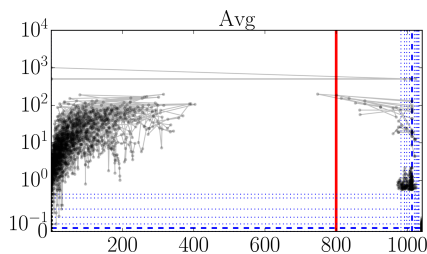
Figure 5. Illustrative plots for visually identifying outliers (see text for an explanation): FINO1 21 m air pressure data (hPa).
