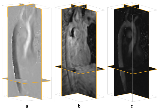
Figure 2: Respectively, one of the three velocity components (inferior to superior) (a), the magnitude (b) and the corresponding signal to noise ratio (c), computed using the method by Friman et al. [FHH*10]. All at peak systole of a healthy volunteer.
