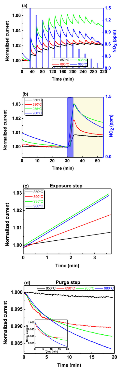
Fig. 5. (a) Real-time behavior of the current of the four sensors upon subsequent NO 2 exposures at different concentrations (blue rectangles). The graphs are normalized to the current value at the gas inlet of the first pulse. (b) Close-up of the first step from panel (a). (c) - (d) Fit of the graphs shown in panel (b) (blue rectangle) and magnification of the decreasing part of the signal recorded during the pulse at 1.5 ppm of NO 2 (yellow rectangle), respectively. The curves are normalized to the value of current at the inlet (c) and stop (d) of the gas flow in the test chamber. Inset: fit of the graphs in the panel (d). As the fit of the black curve (MLG850) does not converge, it is omitted from the Inset.
