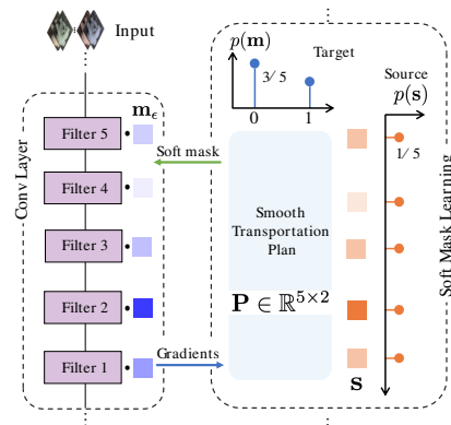
Figure 1. During training we multiply the filters in a layer with soft masks \mathbf{m}_e . The soft masks are obtained by solving an optimal transport problem: minimizing a transportation cost between a uniform source distribution over trainable importance scores \mathbf{s} and a Bernoulli target distribution defined by sparsity ratio i.e. 3/5. During training the soft masks gradually converge to hard masks.
