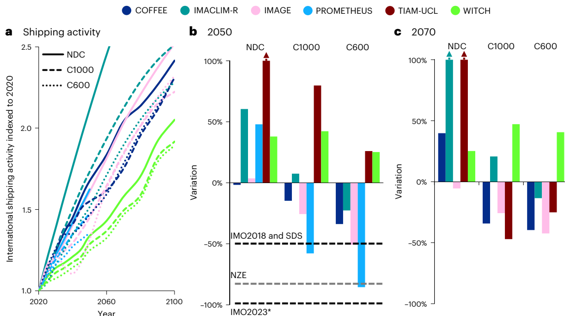
Fig. 3 | International shipping CO 2 emissions. a , International shipping activity level between 2020 and 2100 across scenarios, indexed to 2020. Shipping activity from TIAM-UCL is not shown because the model uses only fuel and efficiency assumptions to project shipping emissions (IMACLIM-R value in 2100: 3.2). b , Variation of the annual CO 2 emissions from international shipping in 2050 when compared with 2020 across scenarios (for clarity, on the y axis we use the range of -100% to +100%, with the arrow indicating that the TIAM-UCL NDC variation is slightly above this range, with a value of 115%). IMO2018 indicates the 50% emission cutback associated with IMO's preliminary strategy 43 (total 2020 international shipping emissions are very close to total 2008 emissions, used as the baseline year for IMO2018), while NZE refers to the IEA's net-zero scenario 57 . IMO2023* indicates a 100% cutback, that is, zero direct international shipping emissions. As discussed, the revised IMO strategy sets a target of achieving
