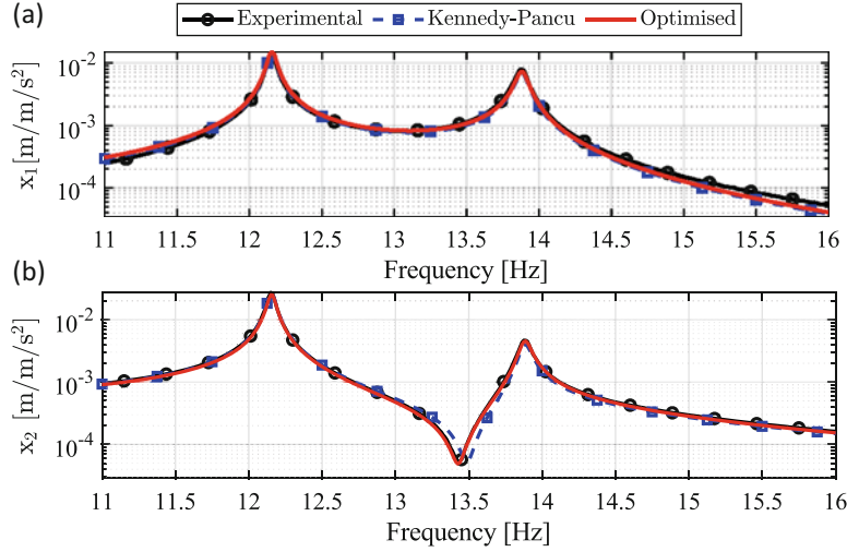
Fig. 28.4 Comparison between the experimental and analytical receptances of the first (a) and the second (b) degree of freedom of the system
