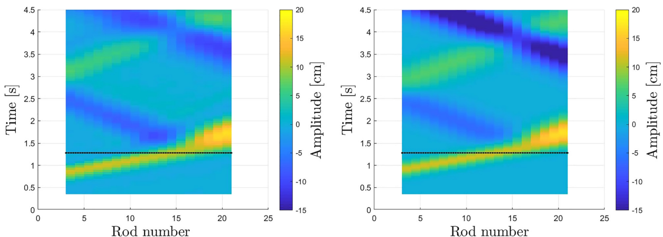
FIG. 4. (Color online) Experimental (left) and simulated (right) wave propagation in space-time. The color map represents the amplitude of the rotation of the bars: the bright yellow 'band' shows the waves with positive amplitude, the darker areas correspond to reflected waves with negative amplitude, while the brightening and the broadening in the vertical direction, starting around t = 1.5 s, represent the period and amplitude increase, respectively. The dotted line shows the time at which the tension in the system is suddenly dropped.
