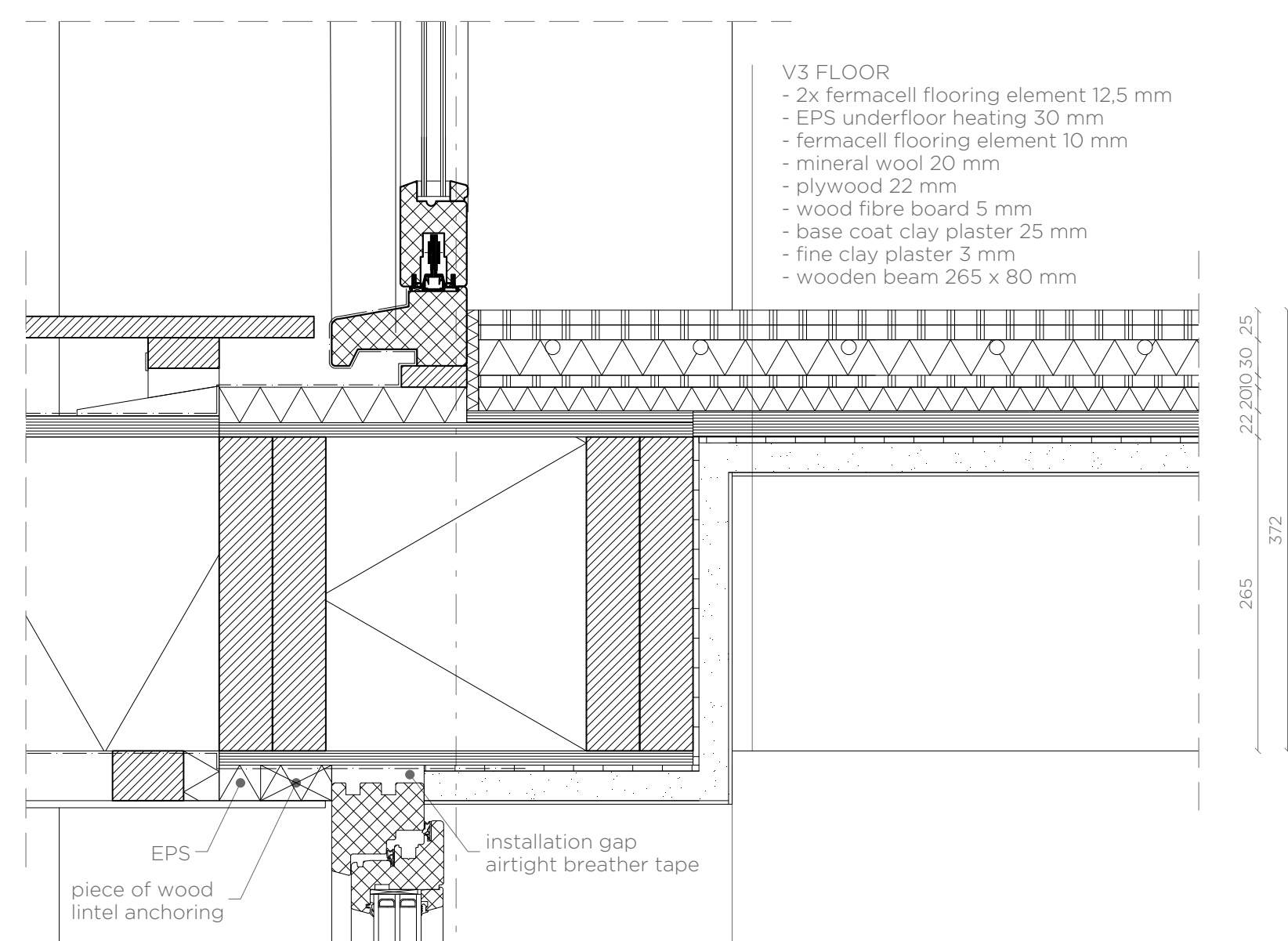
DETAIL V3 - FLOOR
