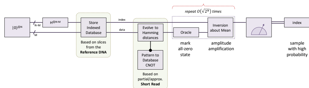
Figure 5. Quantum phone directory algorithm.
