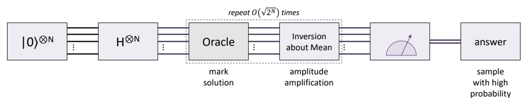
Figure 3. Grover's search steps.
