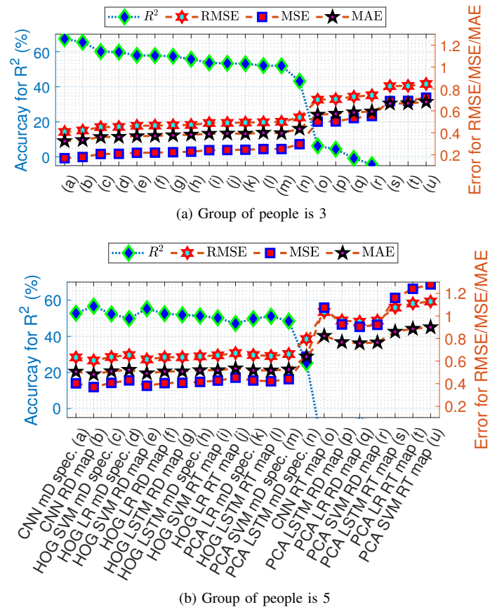
Fig. 2. Regression results shown for different regression models and for three- and five-people groups in (a) and (b), respectively. The considered evaluation metrics are the R^2 score, RMSE, MSE, and MAE.
