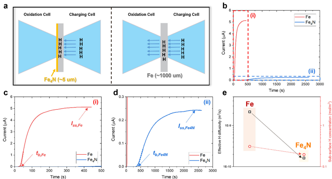
Figure 3. H-cell permeation experiment. a) Schematic illustration of hydrogen permeation experiments of the Fe and as-designed \gamma' -Fe 4 N membranes. b) Hydrogen permeation curves of the Fe (red) and Fe 4 N@Fe (blue). c, d) Enlarged view of dashed red and blue lines in (b), respectively. e) Logarithmic plot of effective hydrogen diffusivity ( D_{\text{eff}} ) and sub-surface H concentration ( C_{0R} ) with the same scale range of Fe and Fe 4 N coated membranes.
