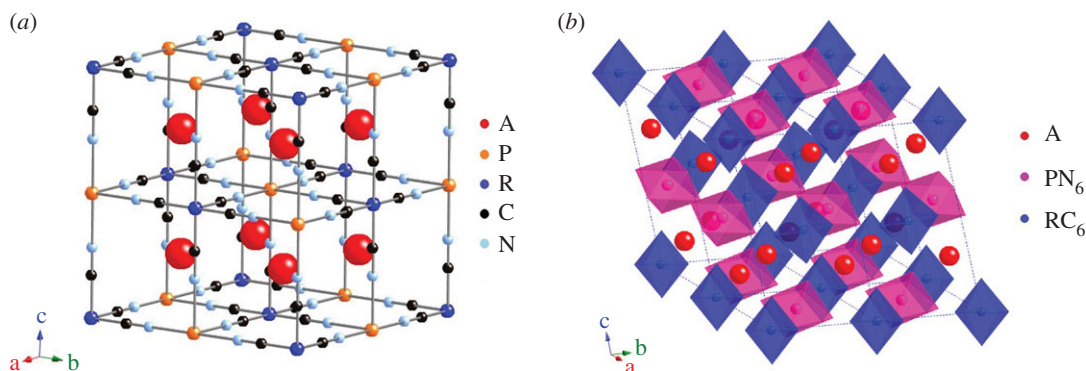
Figure 1. Structure of PBA, A_xP[R(CN)_6]_{1-y} with y = 0 (no vacancies), (a) cubic space group Fm\bar{3}m and (b) monoclinic space group P2_1/c . Water is omitted for clarity. Figures made using CrystalMaker.
