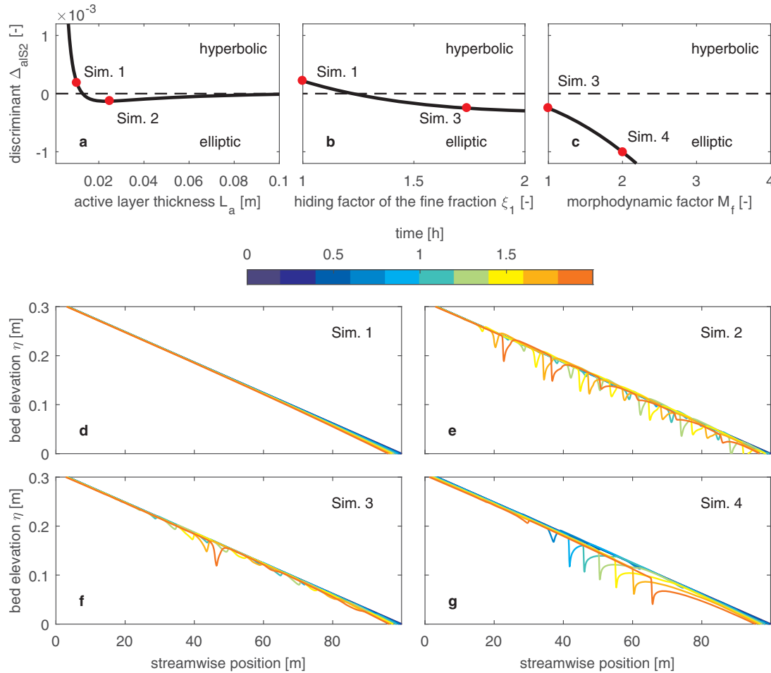
Fig. 4. Discriminant \Delta_{\text{als2}} , Eq. (26), as a function of (a) the active layer thickness L_a , (b) the hiding function of the fine fraction \xi_1 , and (c) the morphological factor M_f . Numerical solutions of (d) Simulation 1, (e) Simulation 2, (f) Simulation 3, and (g) Simulation 4. See Table 3 for the parameters definition.
