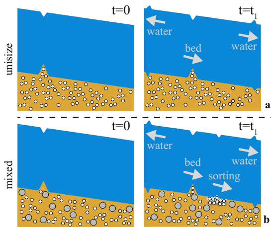
Fig. 1. Schematic of the effect of a perturbation in bed elevation in (a) a unisize sediment case and (b) a mixed sediment case. In the latter case, a perturbation in bed elevation introduces another wave, which is mainly related to the bed surface grain size distribution. Yet, each wave perturbs the flow, bed elevation, and bed surface grain size distribution. The arrows indicate the direction of propagation of the perturbations under subcritical flow conditions. The words “water”, “bed”, and “sorting” refer to a perturbation in water flow, bed level, and surface grain size distribution, respectively.
