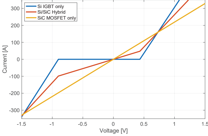
Fig. 5. The on-state characteristics of all three configurations considered in this paper.
