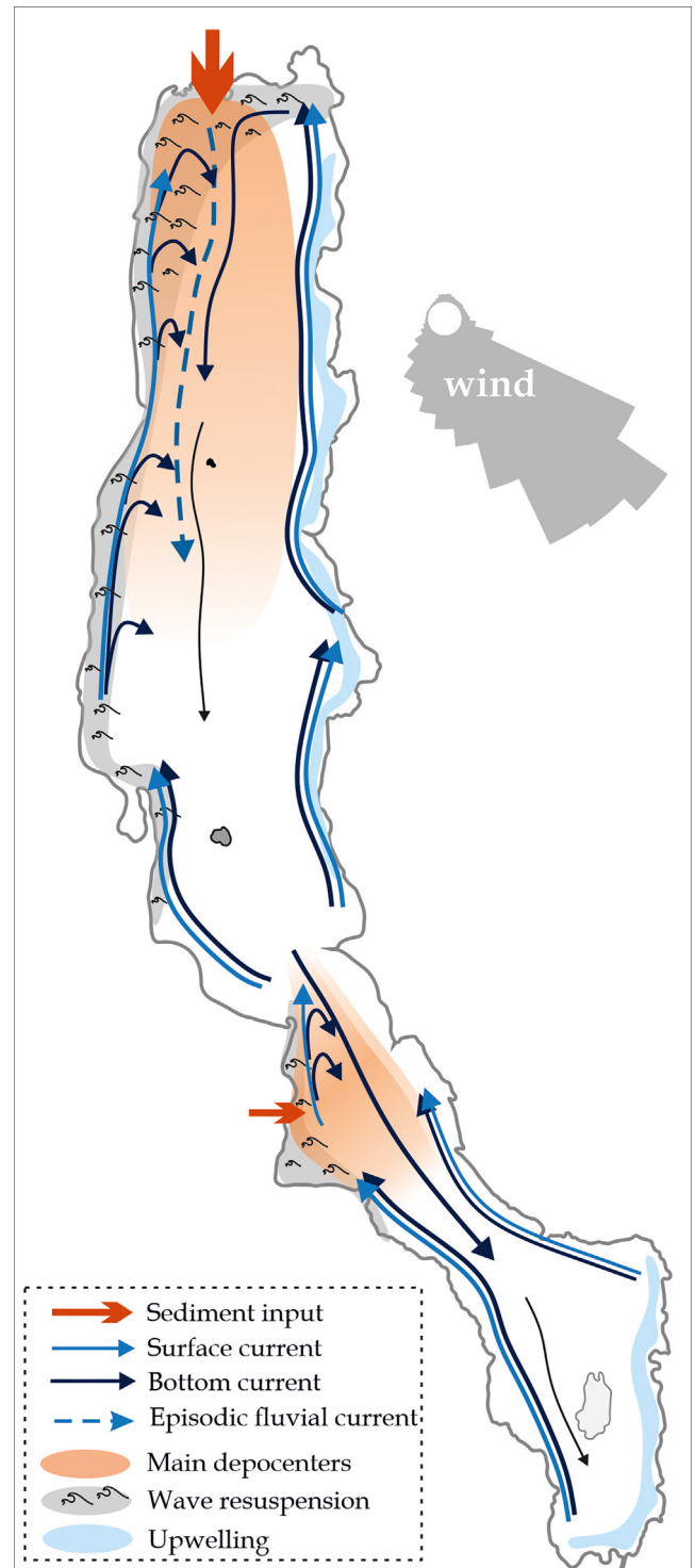
Fig. 11. Conceptual model of hydro-sedimentary dynamics in Lake Turkana based on numerical simulations with Delft3D.
