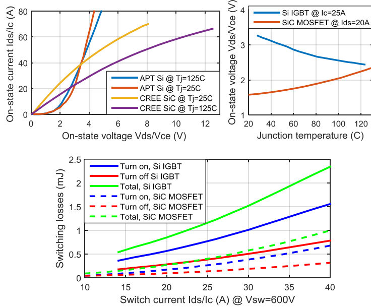
Fig. 9 – Conduction and switching loss characteristics of the APT Si and CREE SiC switch
