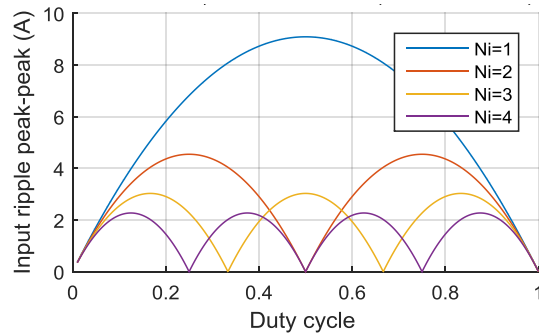
Fig. 3 – Magnitude of input ripple as a function of duty cycle for different number of interleaved stages. V_{dc}=750V , f_{sw}=47kHz , L=443\mu H
