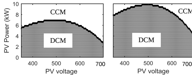
Fig. 7 – Boundary between CCM and DCM using 40 \mu (left) and 26 \mu (right) Kool M \mu core. 26 \mu core inductor has larger operation in DCM.
